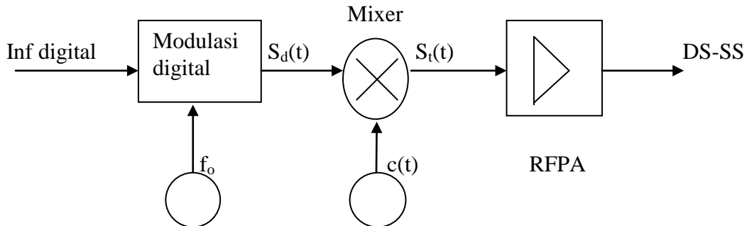
Gambar 4. Prinsip dasar Direct Sequence Spread Spectrum :
