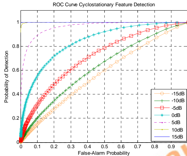
Gambar 3. Grafik Kinerja Cyclostationary Feature Detection
