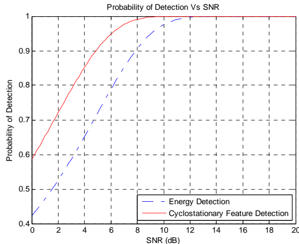
Gambar 10. Probability of False Alarm (PFA) sebesar 0,0001
