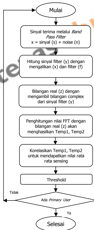
Gambar 2. Diagram Alir Simulasi Cyclostationary Feature Detection
