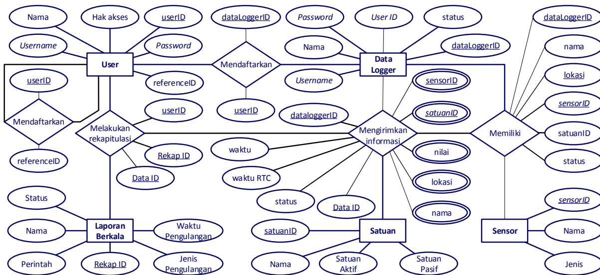
Gambar 6. Entity Relationship Diagram (ERD) sistem
