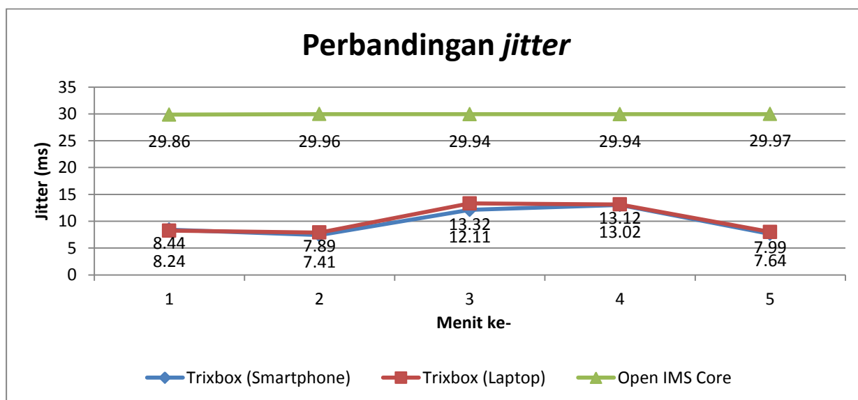
Gambar 3. Perbandingan jitter
